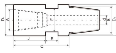
Pin-Box Adapters
